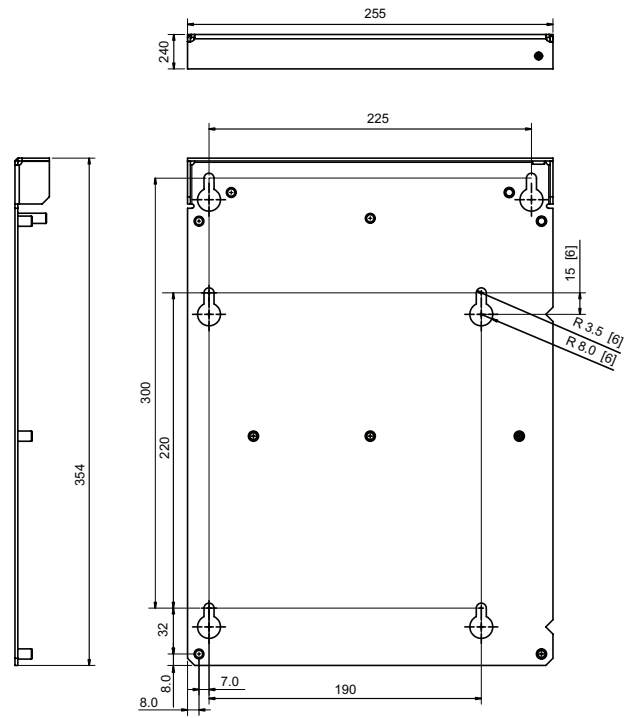
Figure 3.1 Baseplate mounting holes
