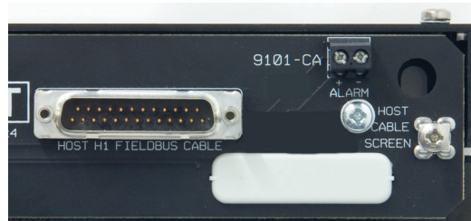
Figure 4.4 Host H1 and ALARM connectors
